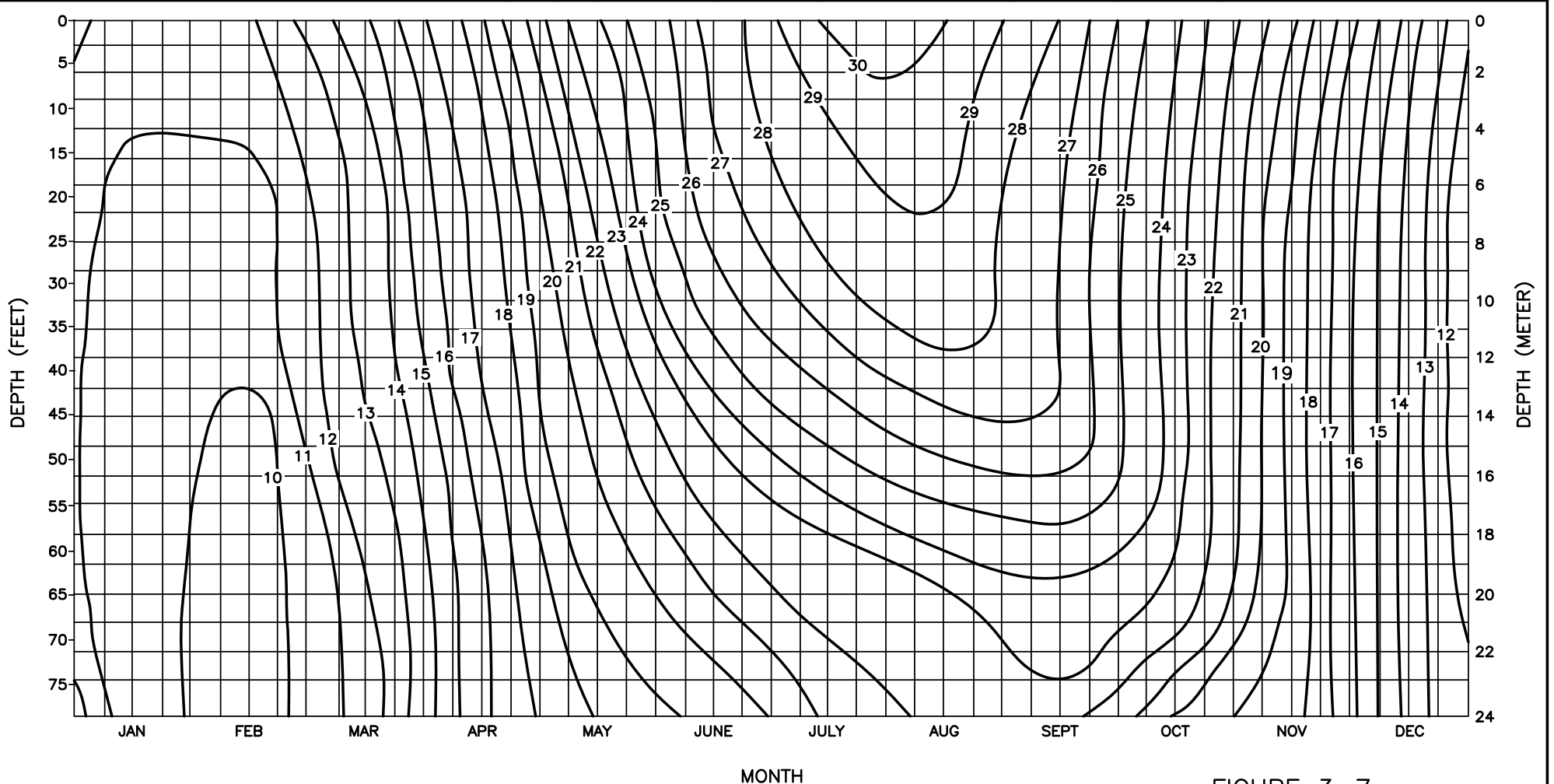
FIGURE 3-7 RESERVOIR TEMPERATURE (C°) TIME HISTORY
